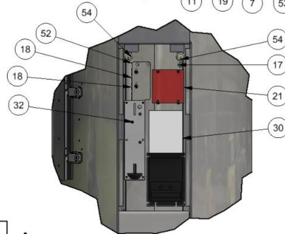
DETAIL C
